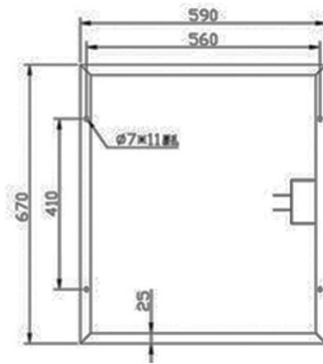
SOLAR PANEL
