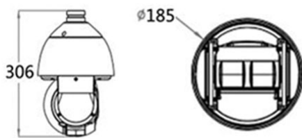
PTZ CAMERA
